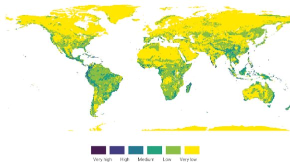
Figure 7: Global STAR Threat Abatement map. Grid cell score categories range from Very Low to Very High. Note that low scores do not mean that there are no threatened species present. Grid cells are at a 5km resolution.
