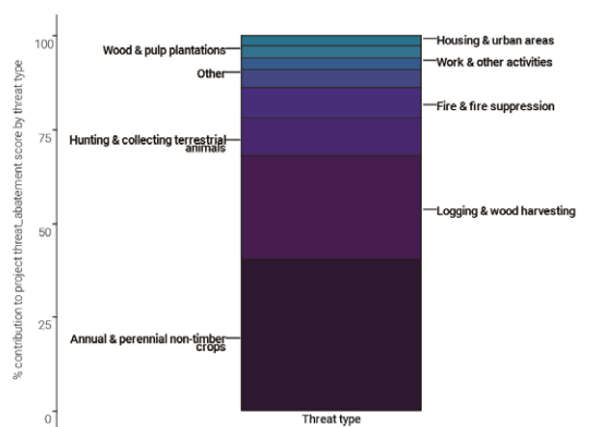
Figure 8: Breakdown of STAR Threat Abatement scores within the Area of Interest by threat type.
