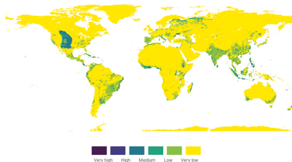
Figure 10: Global STAR Restoration map. Grid cell score categories range from Very Low to Very High. Grid cells are at a 5km resolution.
