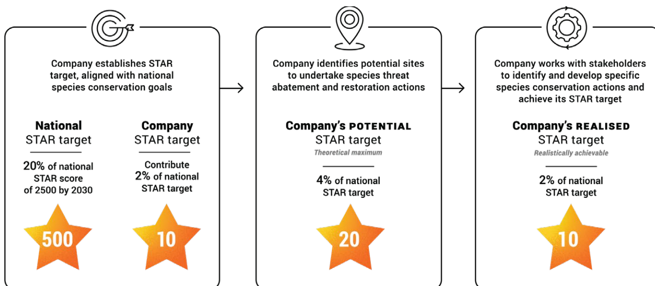
Figure 3: Approach to establishing a STAR target and identifying species threat abatement and restoration actions to achieve the target.
