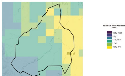
Figure 6: STAR Threat Abatement map for Area of Interest. Grid cell score categories range from Very Low to Very High. Note that low scores do not mean that there are no threatened species present. Grid cells are at a 5km resolution.
