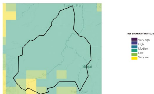
Figure 9: Global STAR Restoration rankings map for Area of Interest. Grid cell score categories range from Very Low to Very High, and reflect the range of values found within the site in the global context. Grid cells are at a 5km resolution.
