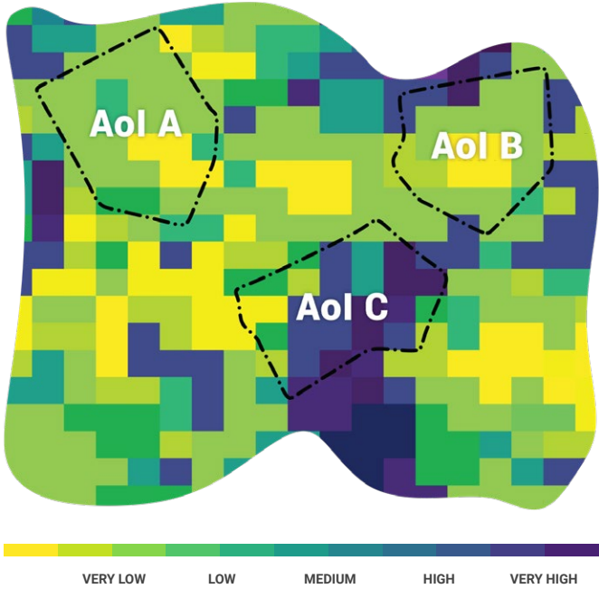
Figure 4: Potential sites (Aols) in the landscape for undertaken threat abatement activities, based on the Potential STAR T (estimate) layer.
