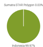
Figure 3: % contribution of total STAR Threat Abatement score for Area of Interest to total country score.
