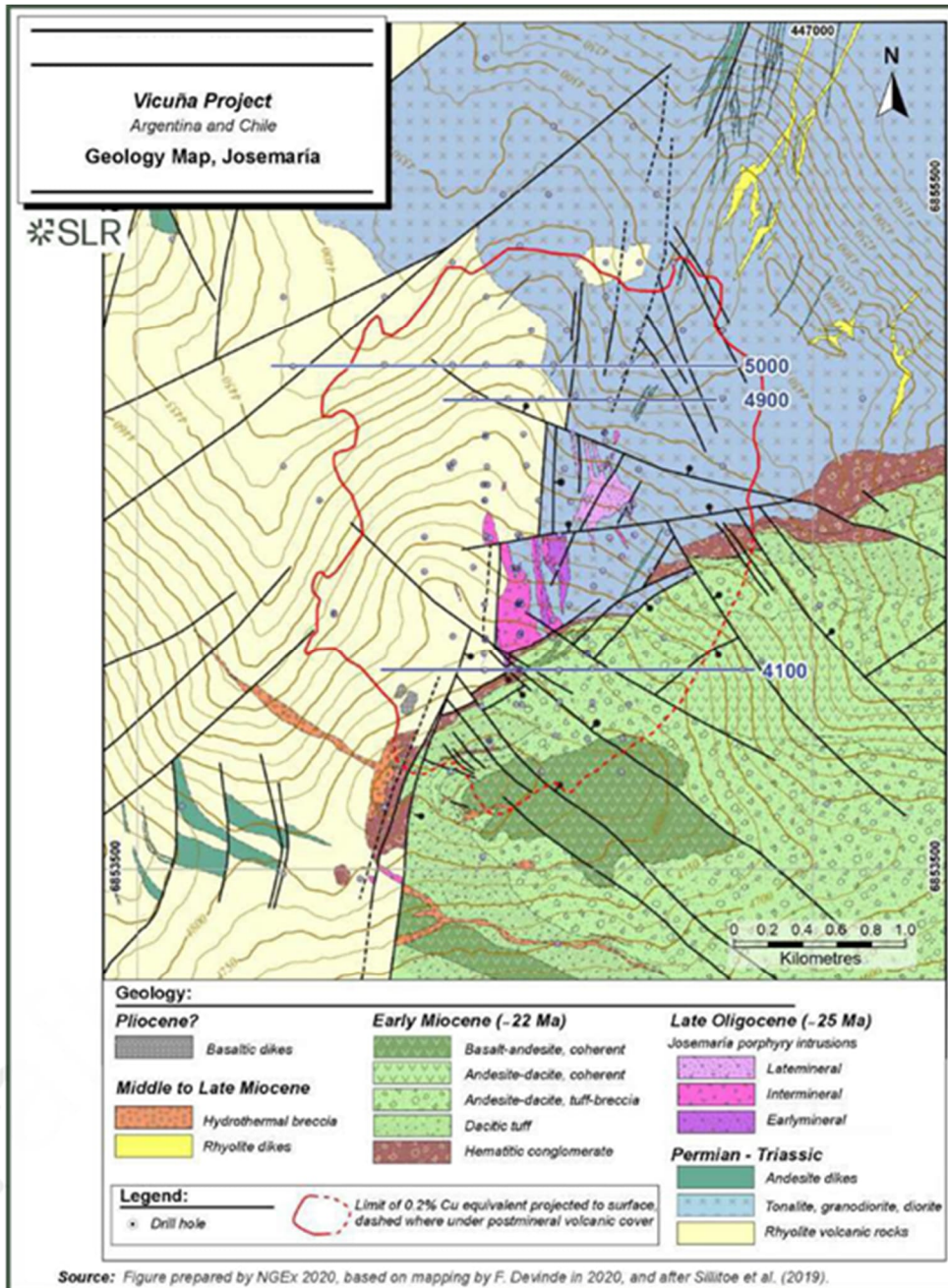
Figure 3-4: Deposit geological map, Josemaria.
