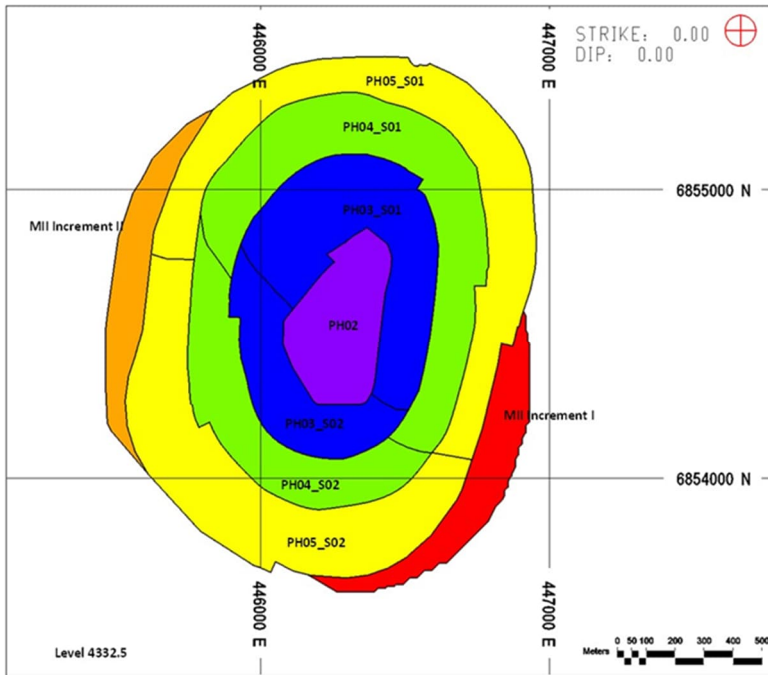
Figure 4-2: Josemaria pit phasing plan view (colours represent different pit phases)
