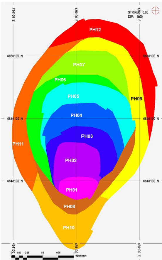
Figure 4-3: Filo pit phasing Planview (colours represent different pit phases)
