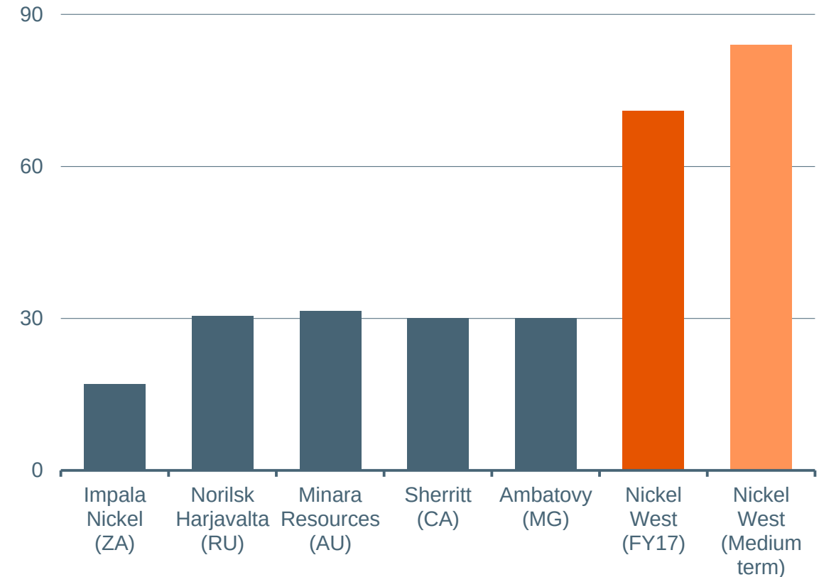
Potential to debottleneck refinery capacity (Capacity, ktpa)
