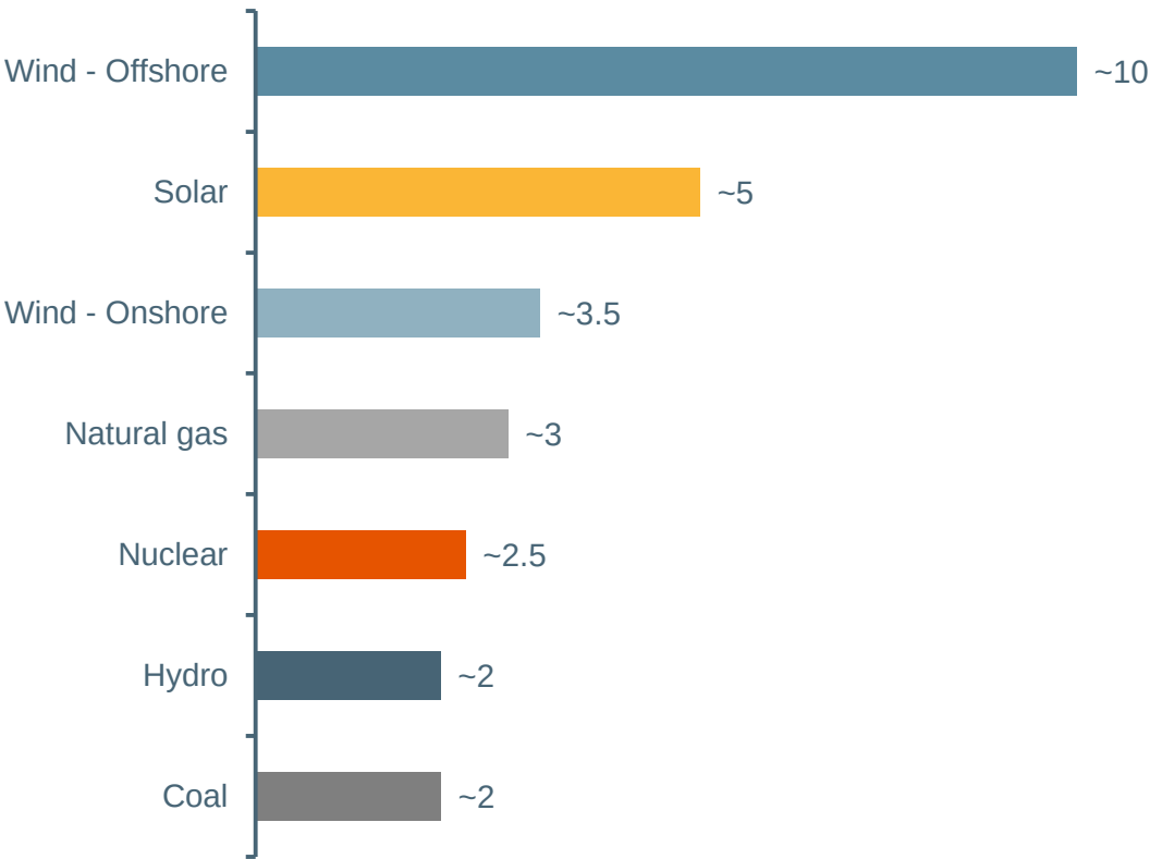
Cu intensity by power generation type (kg/KW)
