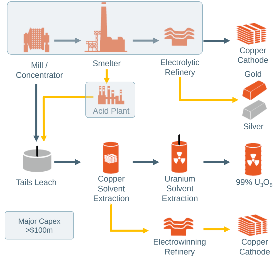
Simplified BFX flowsheet
